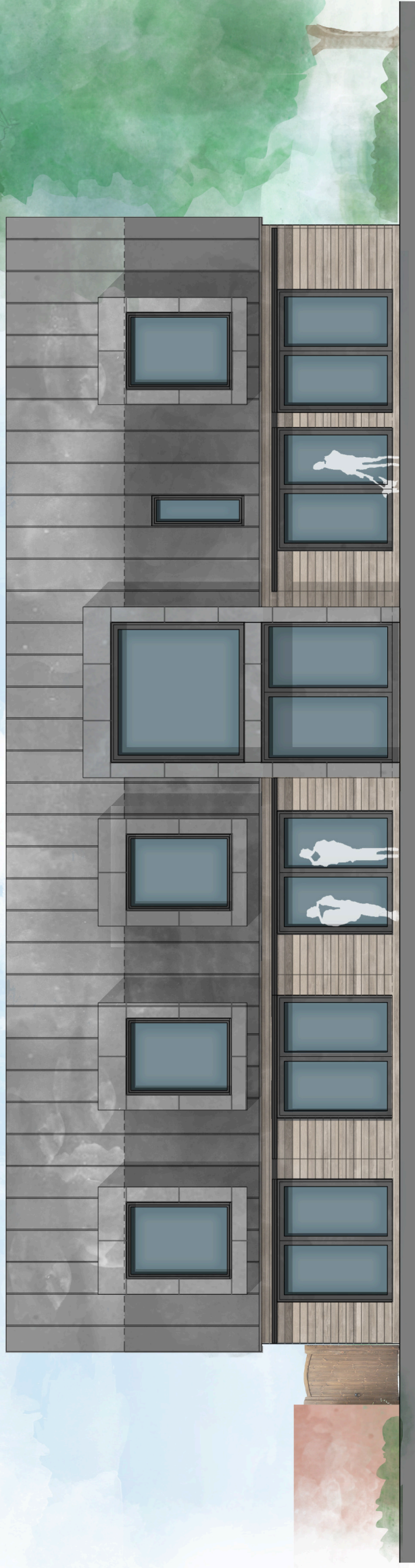
SOUTH-EAST ELEVATION
